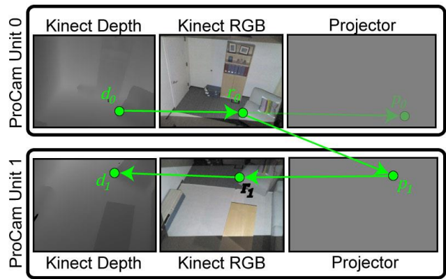
Figure 4. To compute correspondences between two units ( Unit 0 and Unit 1 ), we map a depth pixel in Unit 0 ( d_0 ), to an RGB pixel in Unit 0 ( r_0 ). Next, we look up the corresponding projector pixel in Unit 1 ( p_1 ), via the decoded Gray codes. We then invert the Gray code correspondences to look up the RGB pixel in Unit 1 ( r_1 ). Finally, we invert the Kinect’s transfer map resulting in depth pixel ( d_1 ).
